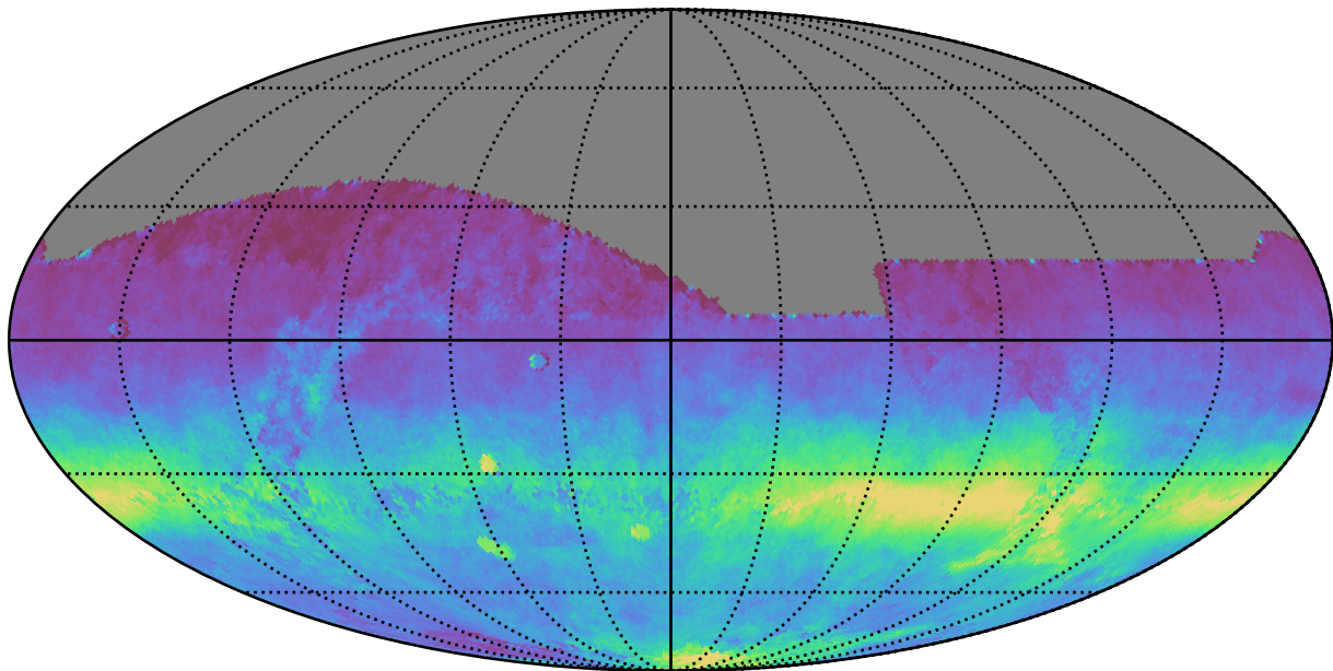
too_10_1v3.4_10yrs All sky all bands: AngleRms rotSkyPos
