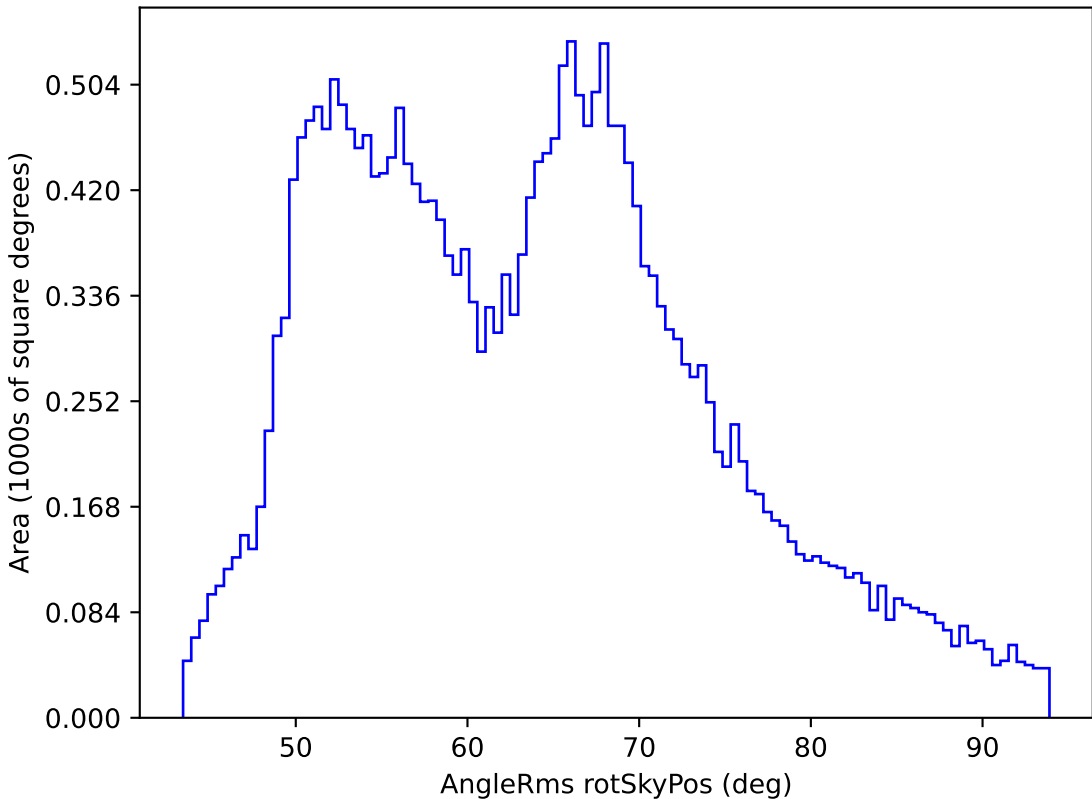
too_10_1v3.4_10yrs All sky all bands: AngleRms rotSkyPos
