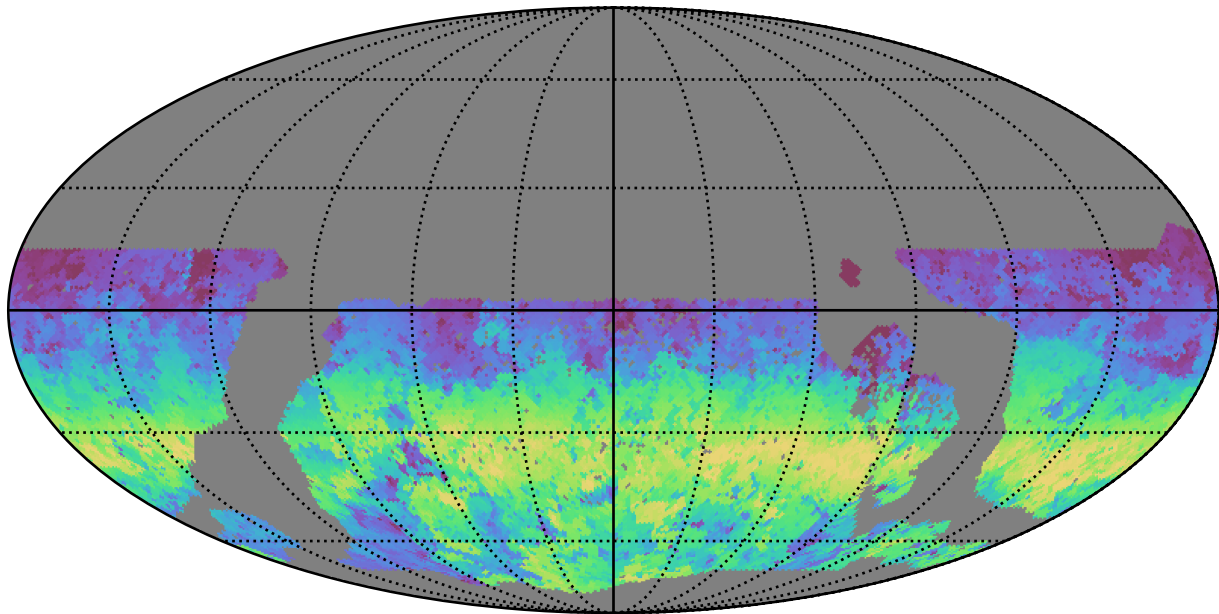
too_10_1v3.4_10yrs WFD u band: AngleRange rotSkyPos
