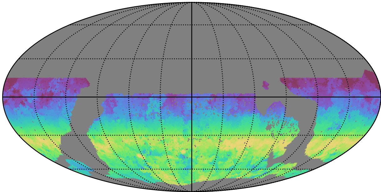
too_10_1v3.4_10yrs WFD r band: AngleRange rotSkyPos
