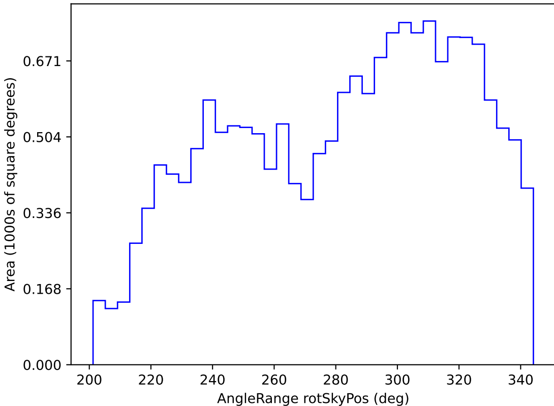
too_10_1v3.4_10yrs WFD r band: AngleRange rotSkyPos
