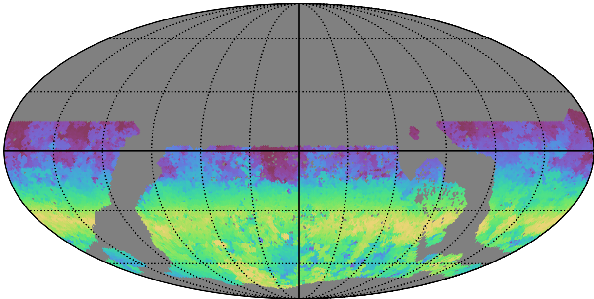
too_10_1v3.4_10yrs WFD g band: AngleRange rotSkyPos
