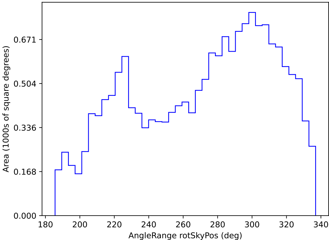
too_10_1v3.4_10yrs WFD g band: AngleRange rotSkyPos
