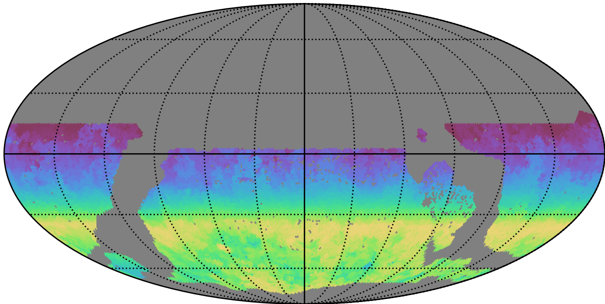
too_10_1v3.4_10yrs WFD all bands: AngleRange rotSkyPos
