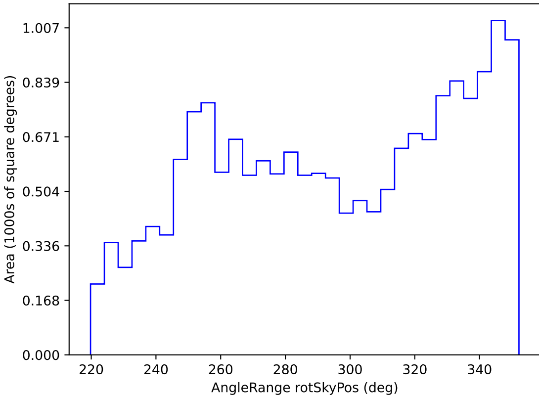
too_10_1v3.4_10yrs WFD all bands: AngleRange rotSkyPos
