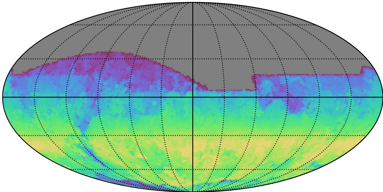
too_10_1v3.4_10yrs All sky z band: AngleRange rotSkyPos
