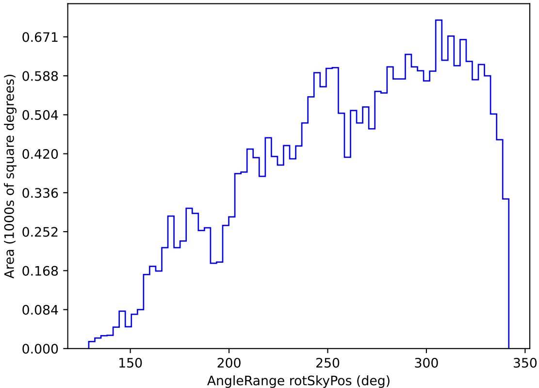
too_10_1v3.4_10yrs All sky z band: AngleRange rotSkyPos
