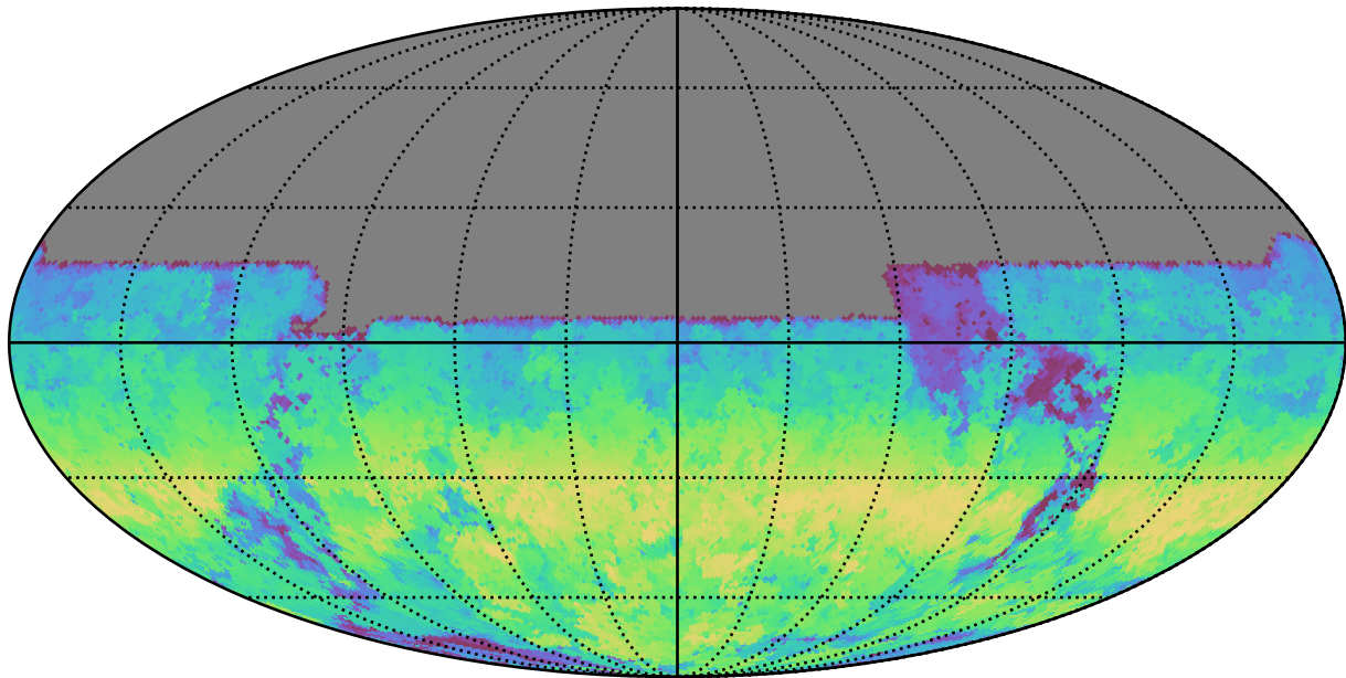
too_10_1v3.4_10yrs All sky u band: AngleRange rotSkyPos
