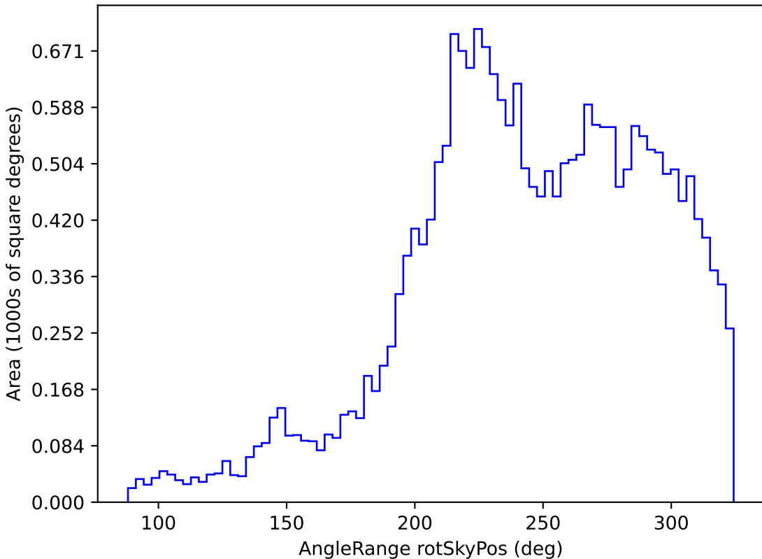
too_10_1v3.4_10yrs All sky u band: AngleRange rotSkyPos
