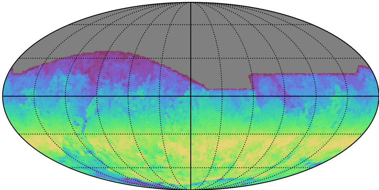
too_10_1v3.4_10yrs All sky i band: AngleRange rotSkyPos
