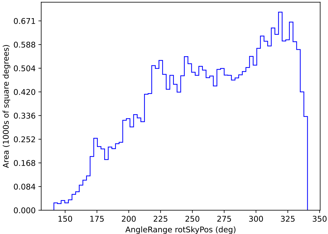
too_10_1v3.4_10yrs All sky i band: AngleRange rotSkyPos
