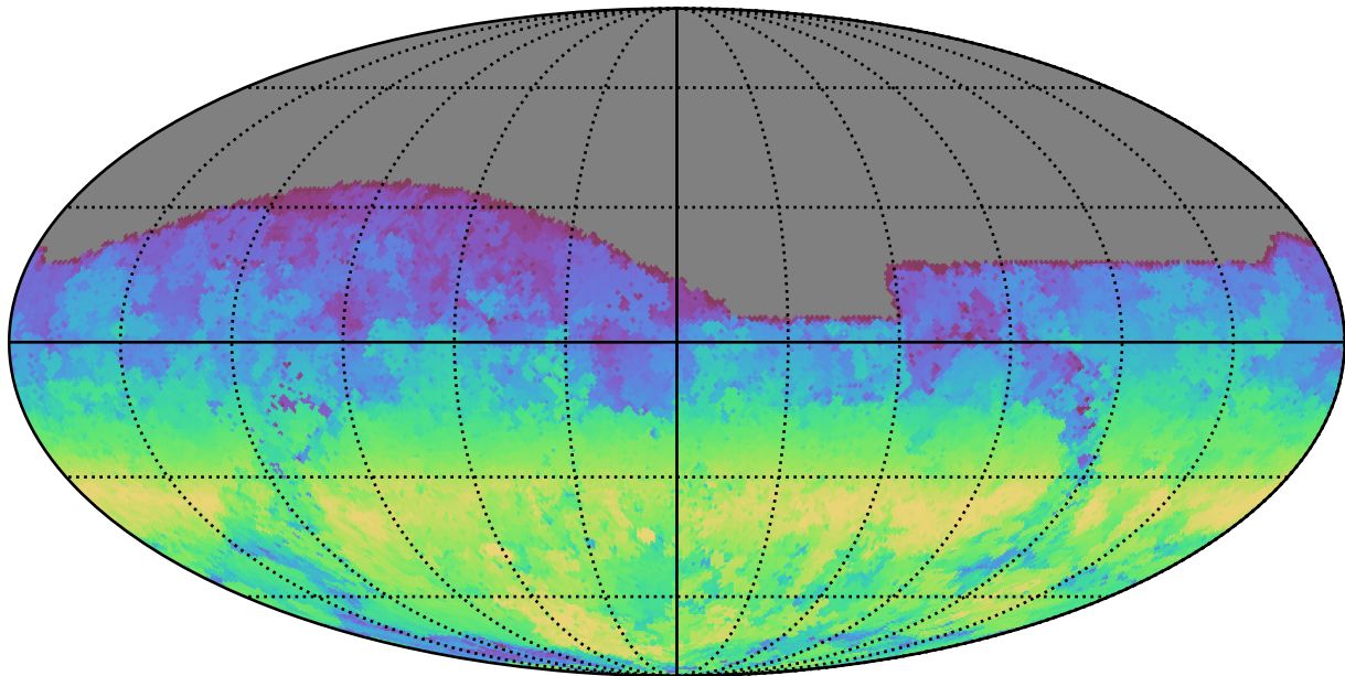
too_10_1v3.4_10yrs All sky g band: AngleRange rotSkyPos
