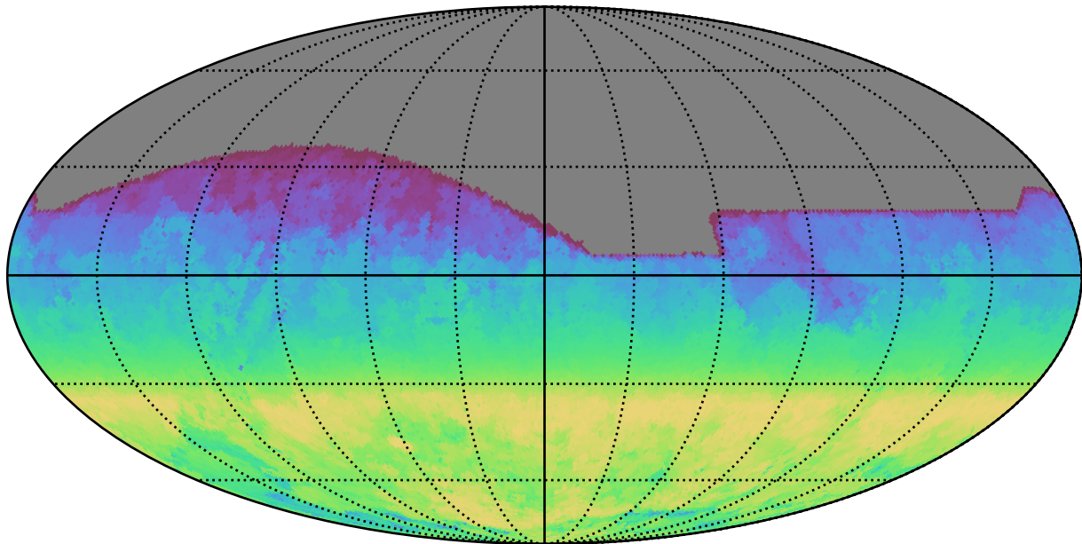
too_10_1v3.4_10yrs All sky all bands: AngleRange rotSkyPos
