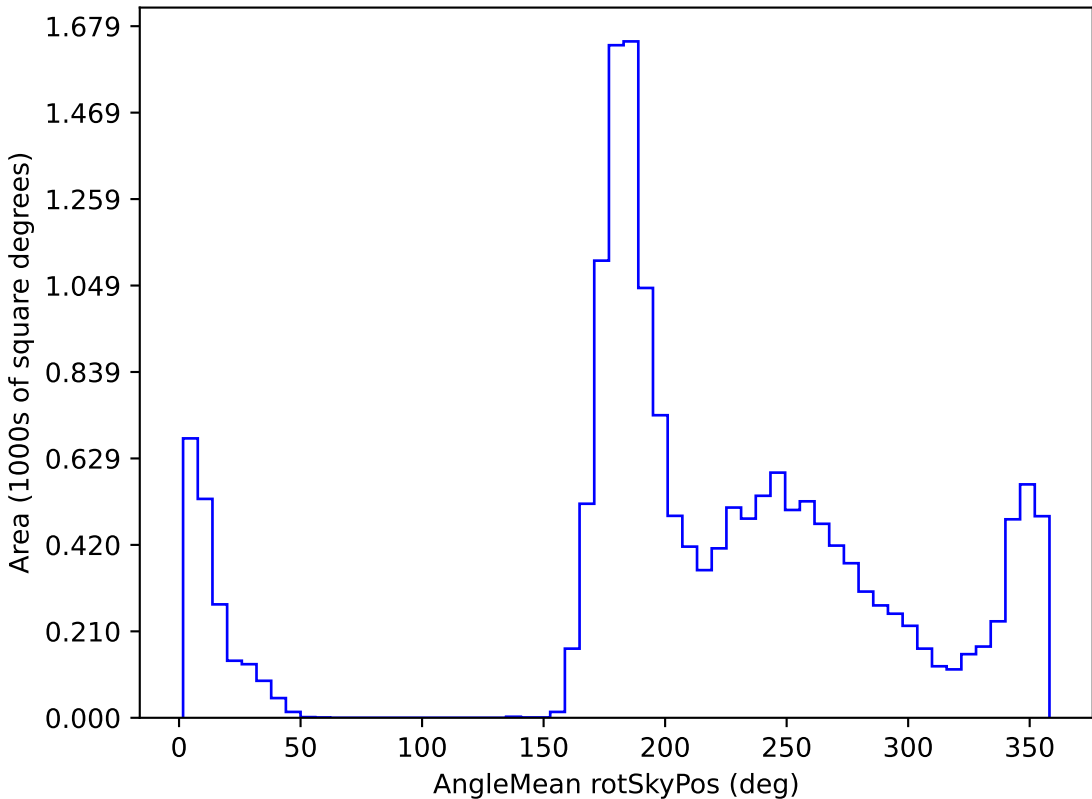
too_10_1v3.4_10yrs WFD z band: AngleMean rotSkyPos
