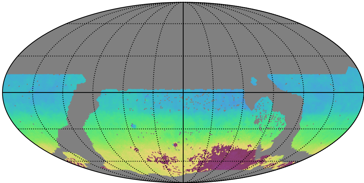
too_10_1v3.4_10yrs WFD y band: AngleMean rotSkyPos
