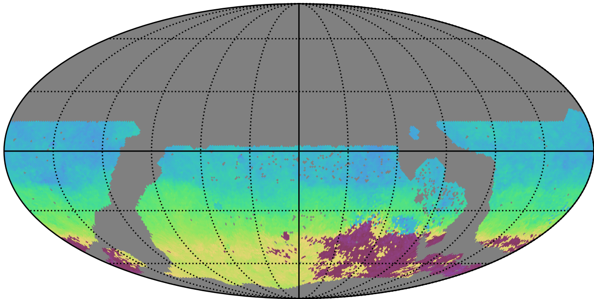
too_10_1v3.4_10yrs WFD u band: AngleMean rotSkyPos
