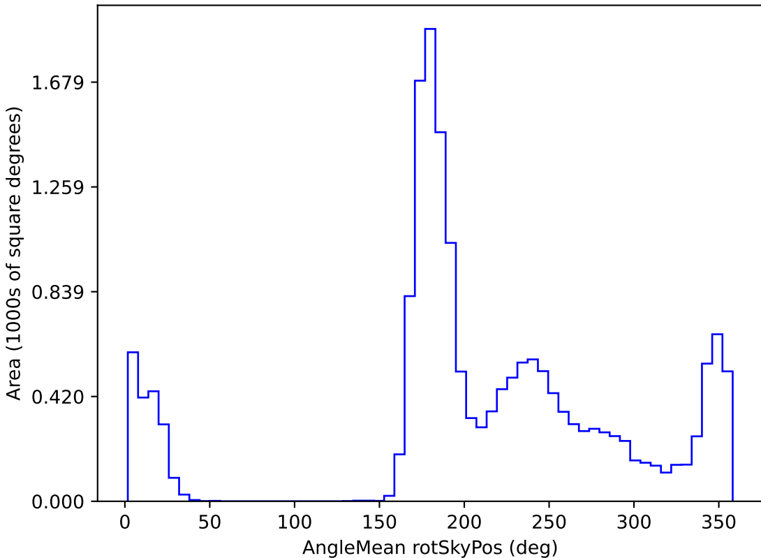
too_10_1v3.4_10yrs WFD r band: AngleMean rotSkyPos
