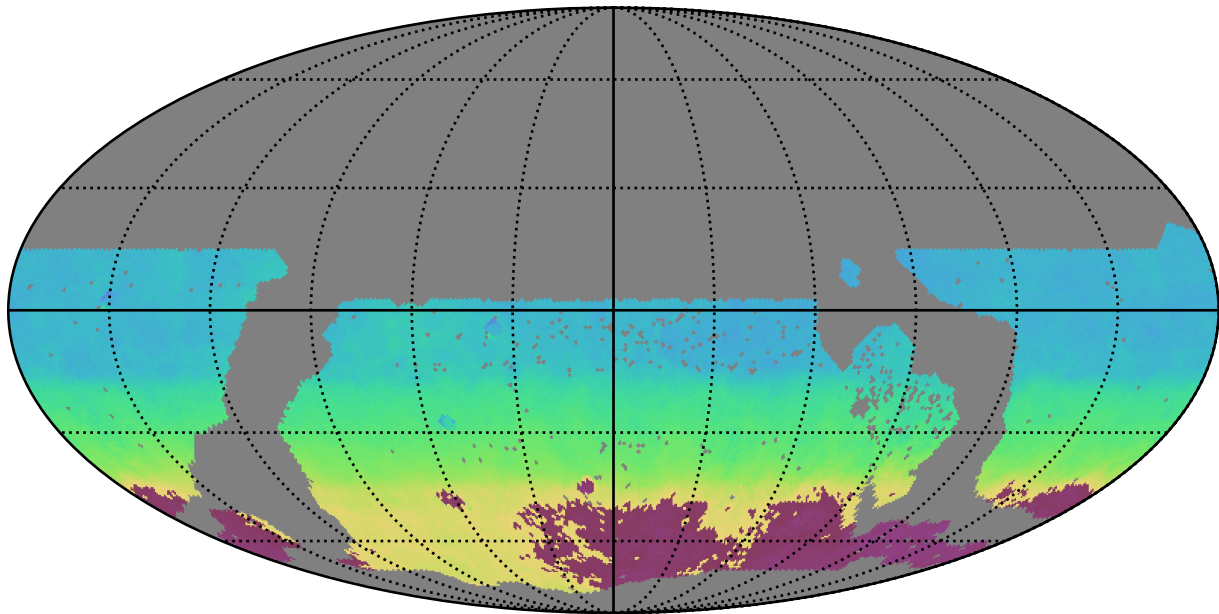
too_10_1v3.4_10yrs WFD i band: AngleMean rotSkyPos
