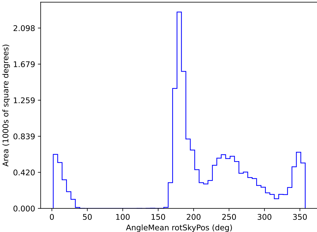
too_10_1v3.4_10yrs WFD i band: AngleMean rotSkyPos
