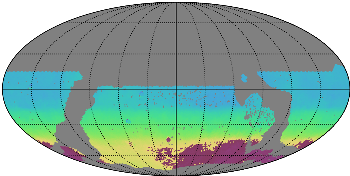
too_10_1v3.4_10yrs WFD all bands: AngleMean rotSkyPos
