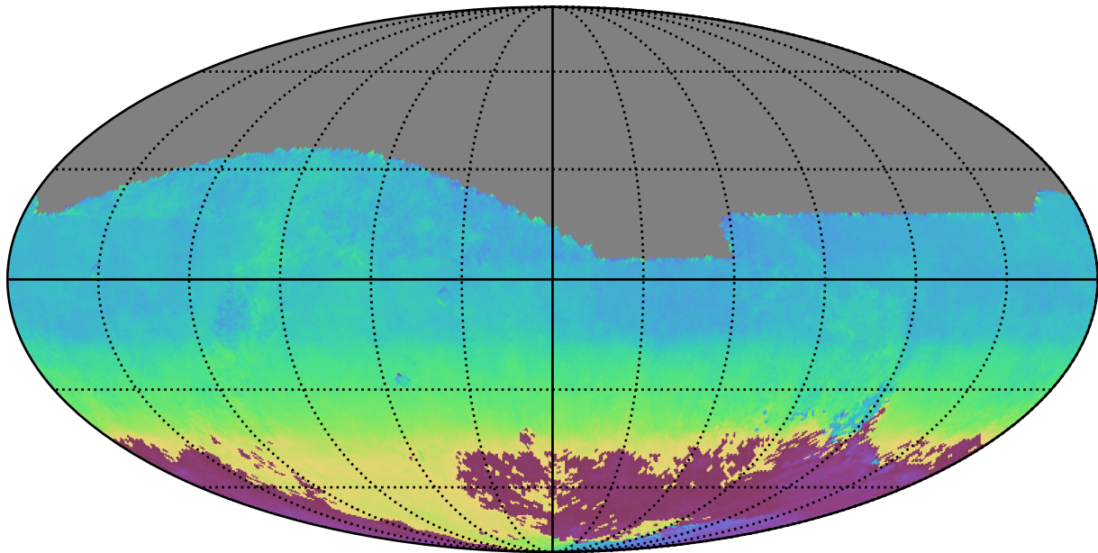
too_10_1v3.4_10yrs All sky z band: AngleMean rotSkyPos
