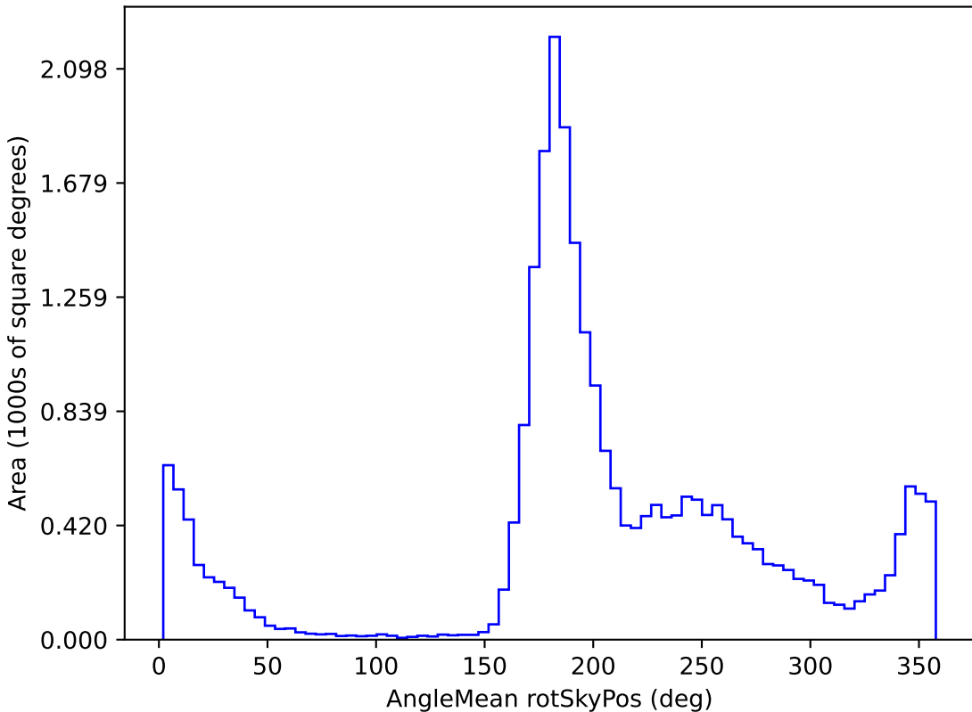
too_10_1v3.4_10yrs All sky z band: AngleMean rotSkyPos
