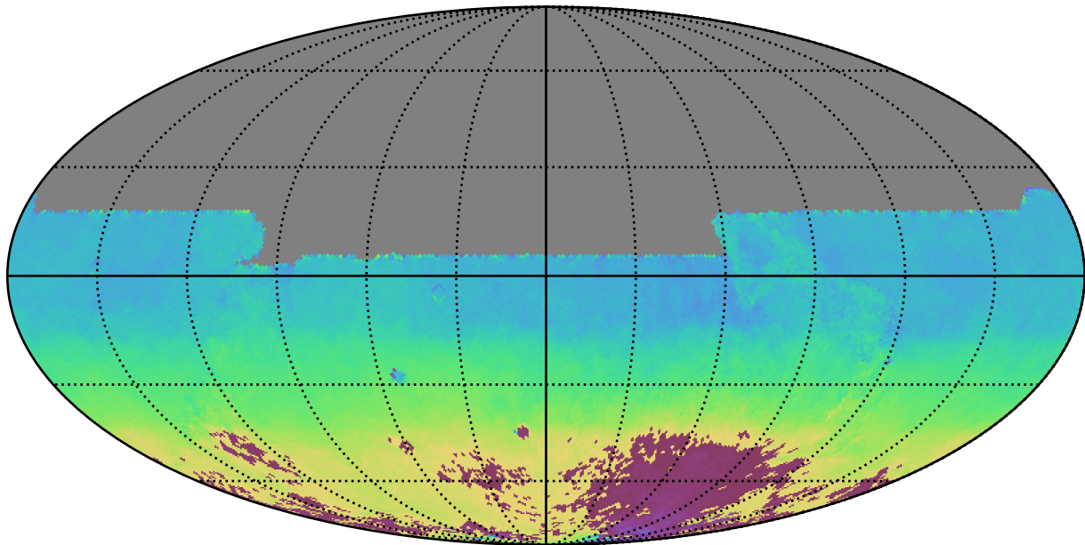
too_10_1v3.4_10yrs All sky y band: AngleMean rotSkyPos
