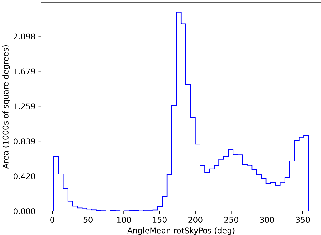
too_10_1v3.4_10yrs All sky y band: AngleMean rotSkyPos
