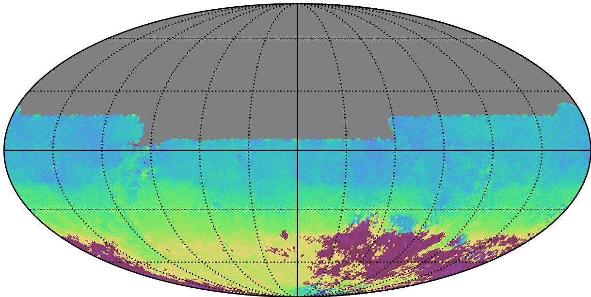
too_10_1v3.4_10yrs All sky u band: AngleMean rotSkyPos
