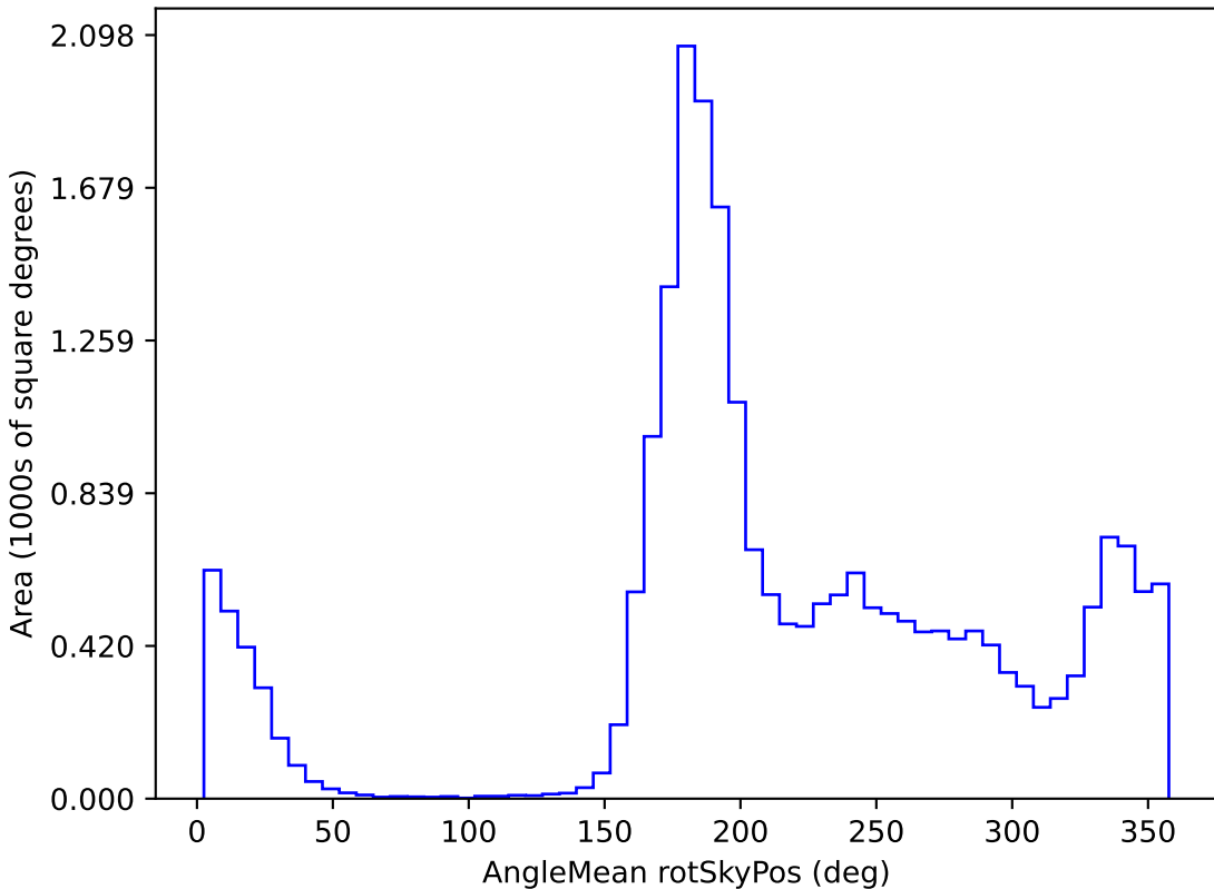
too_10_1v3.4_10yrs All sky u band: AngleMean rotSkyPos
