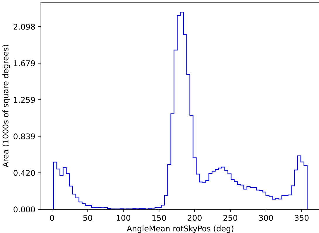
too_10_1v3.4_10yrs All sky r band: AngleMean rotSkyPos
