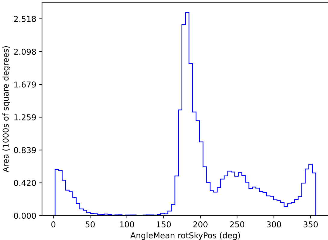
too_10_1v3.4_10yrs All sky i band: AngleMean rotSkyPos
