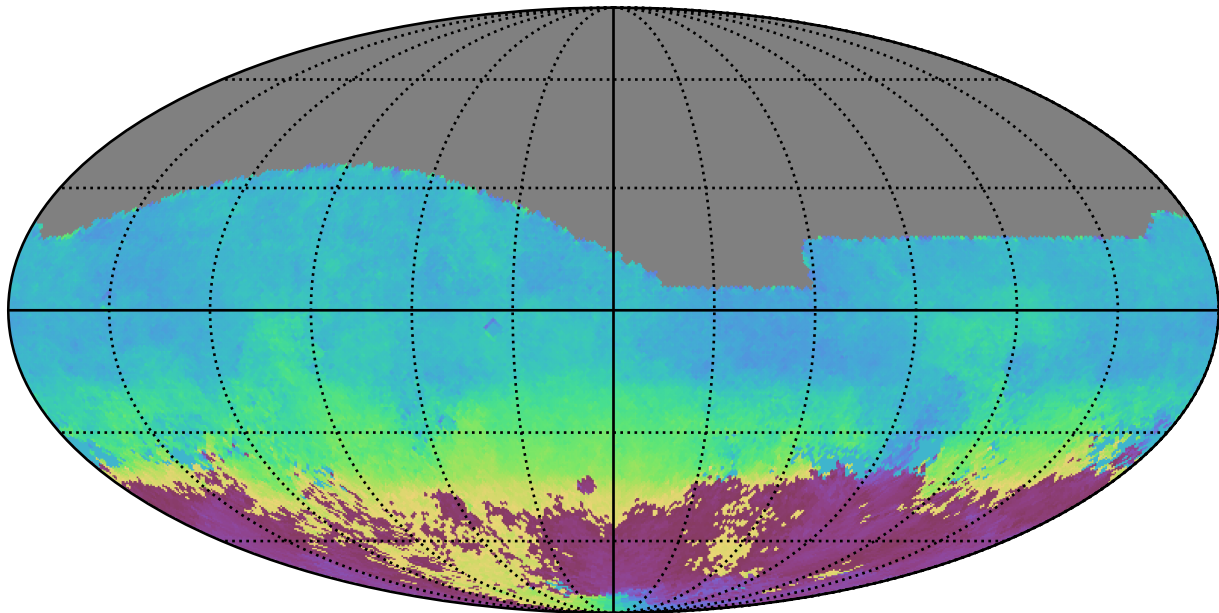
too_10_1v3.4_10yrs All sky g band: AngleMean rotSkyPos
