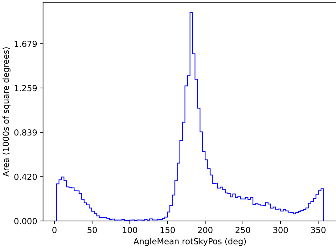
too_10_1v3.4_10yrs All sky g band: AngleMean rotSkyPos
