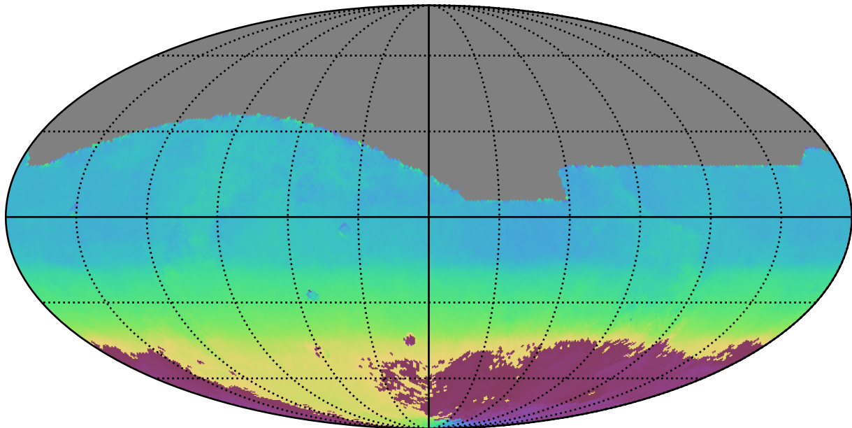
too_10_1v3.4_10yrs All sky all bands: AngleMean rotSkyPos
