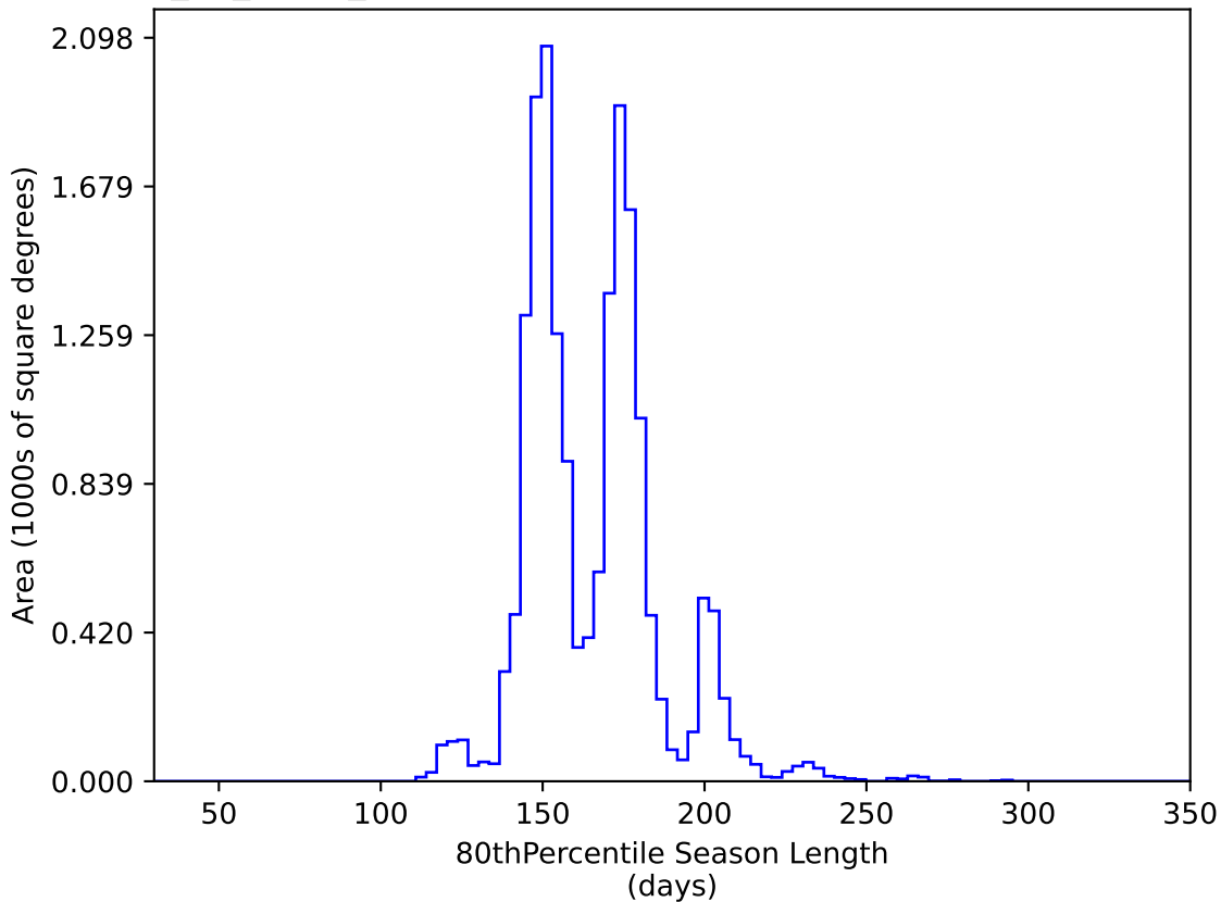
too_10_1v3.4_10yrs WFD y band: 80thPercentile Season Length
