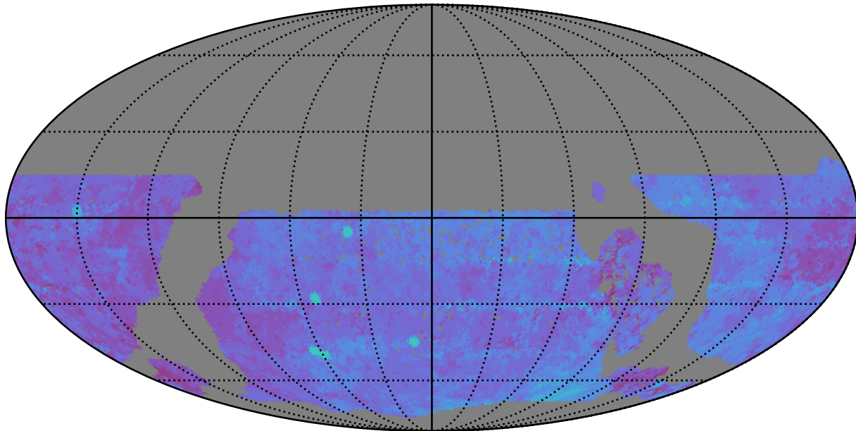
too_10_1v3.4_10yrs WFD u band: 80thPercentile Season Length
