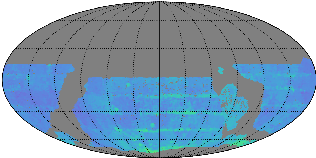
too_10_1v3.4_10yrs WFD r band: 80thPercentile Season Length
