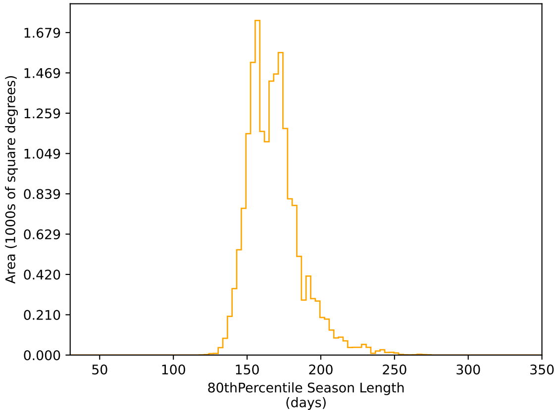
too_10_1v3.4_10yrs WFD r band: 80thPercentile Season Length
