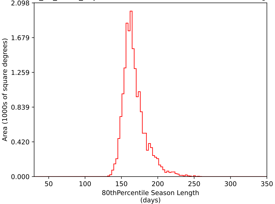
too_10_1v3.4_10yrs WFD i band: 80thPercentile Season Length
