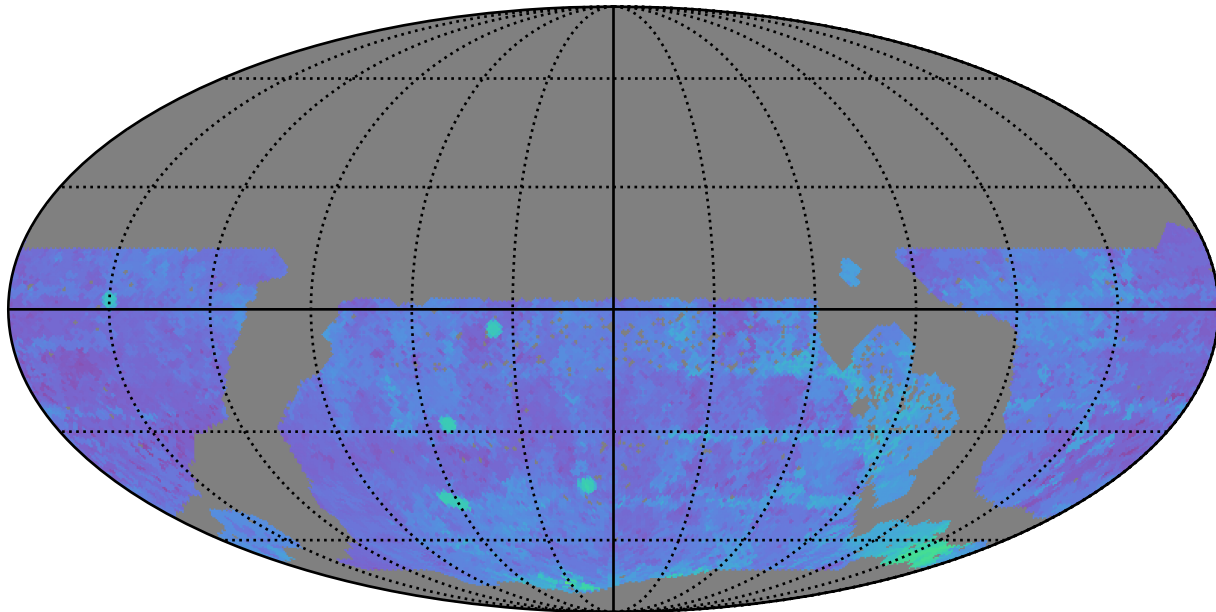
too_10_1v3.4_10yrs WFD g band: 80thPercentile Season Length
