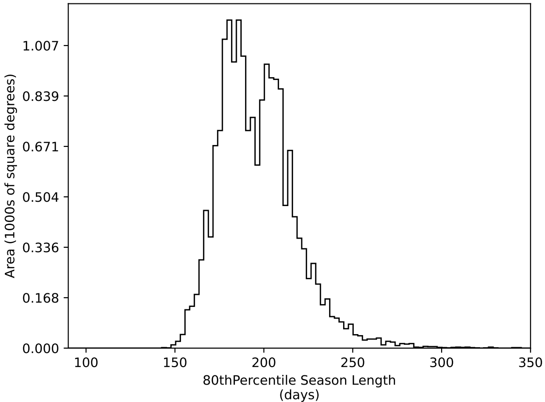
too_10_1v3.4_10yrs WFD all bands: 80thPercentile Season Length
