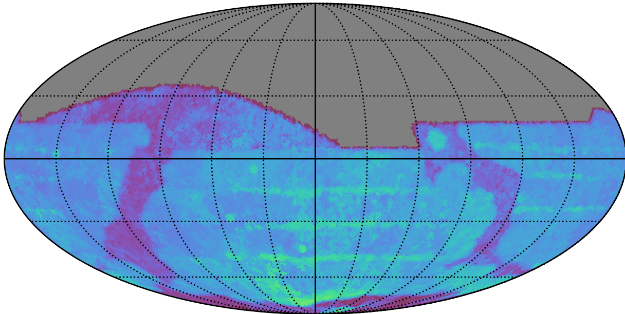
too_10_1v3.4_10yrs All sky z band: 80thPercentile Season Length
