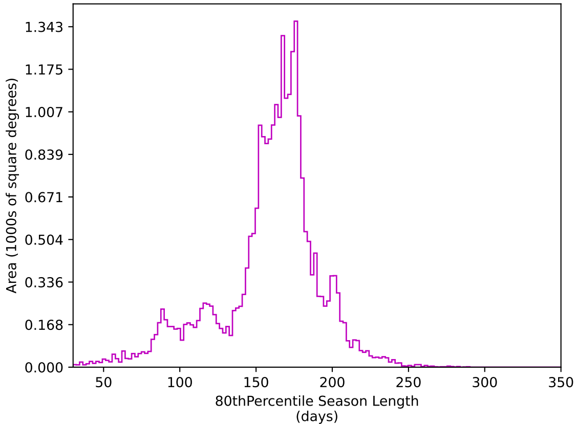
too_10_1v3.4_10yrs All sky z band: 80thPercentile Season Length
