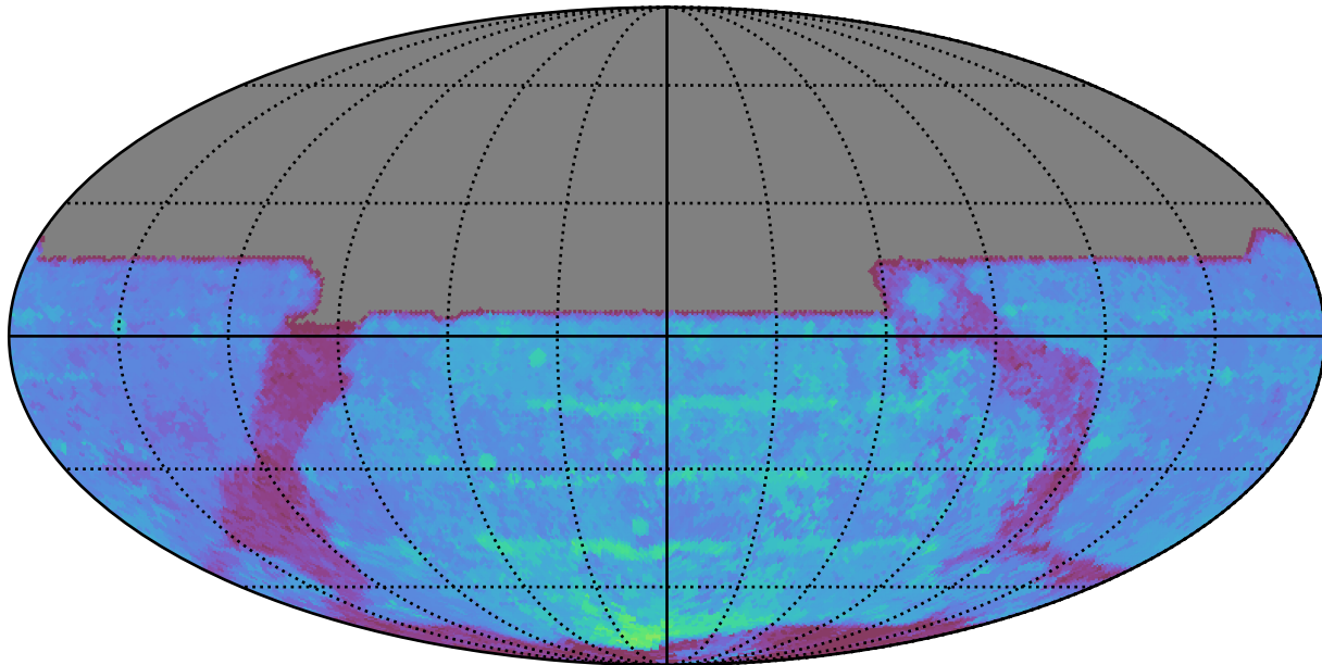
too_10_1v3.4_10yrs All sky y band: 80thPercentile Season Length
