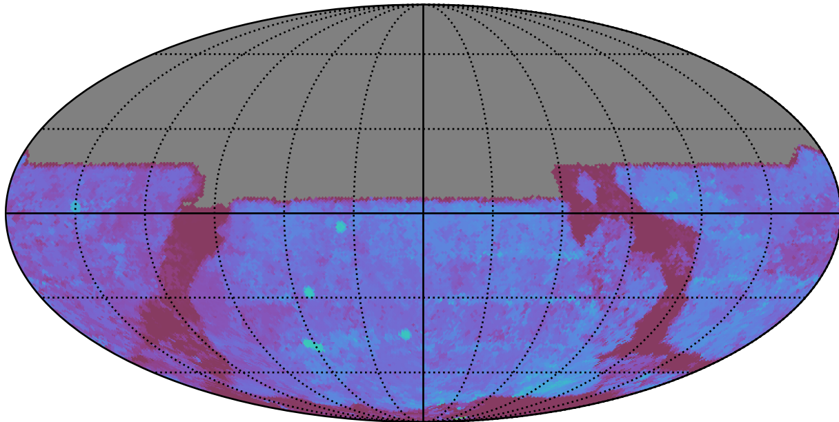
too_10_1v3.4_10yrs All sky u band: 80thPercentile Season Length
