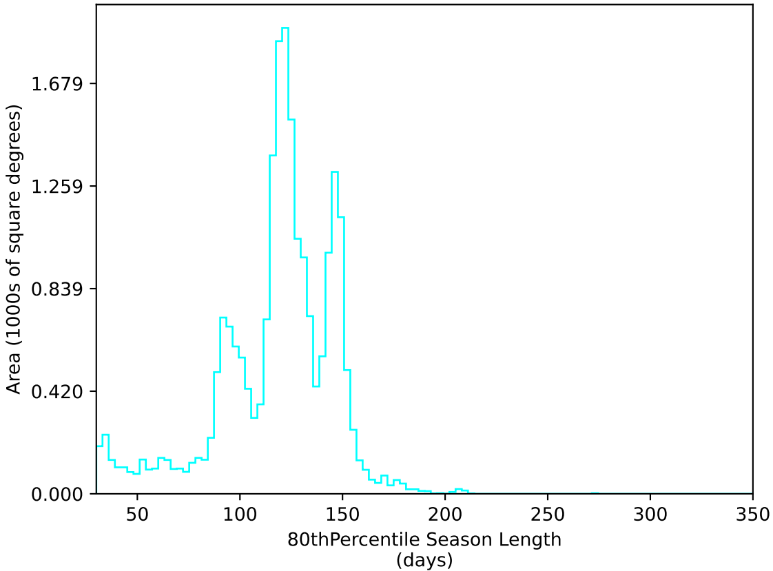
too_10_1v3.4_10yrs All sky u band: 80thPercentile Season Length
