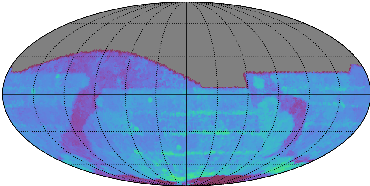
too_10_1v3.4_10yrs All sky r band: 80thPercentile Season Length
