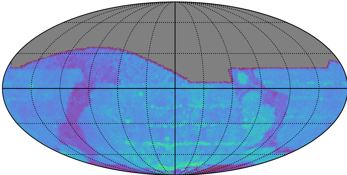
too_10_1v3.4_10yrs All sky i band: 80thPercentile Season Length
