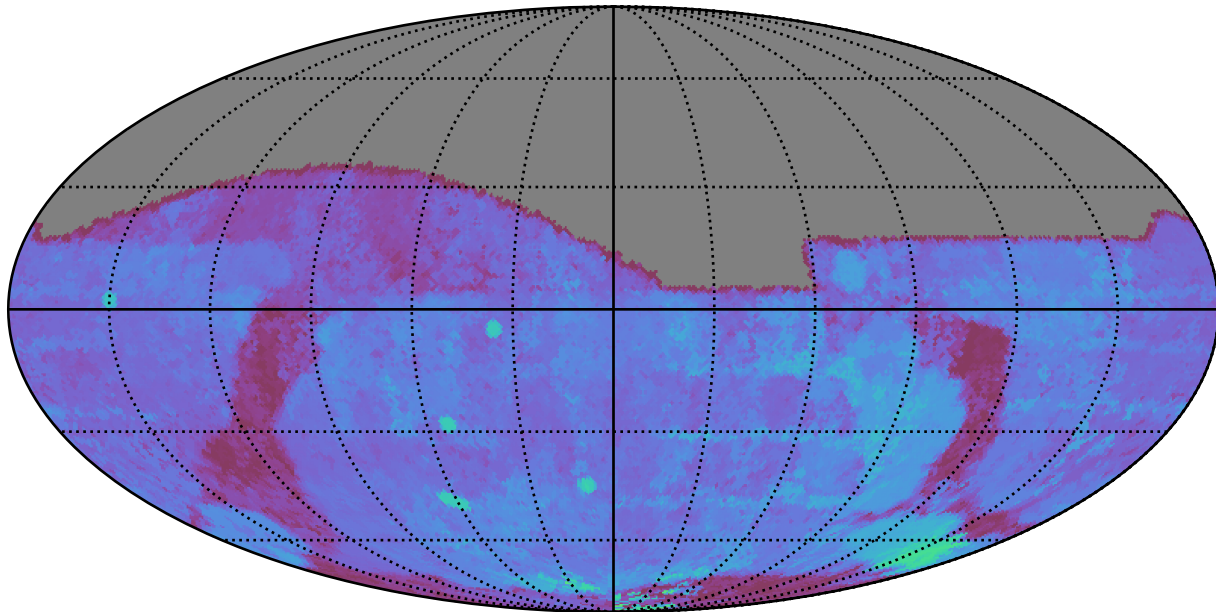
too_10_1v3.4_10yrs All sky g band: 80thPercentile Season Length
